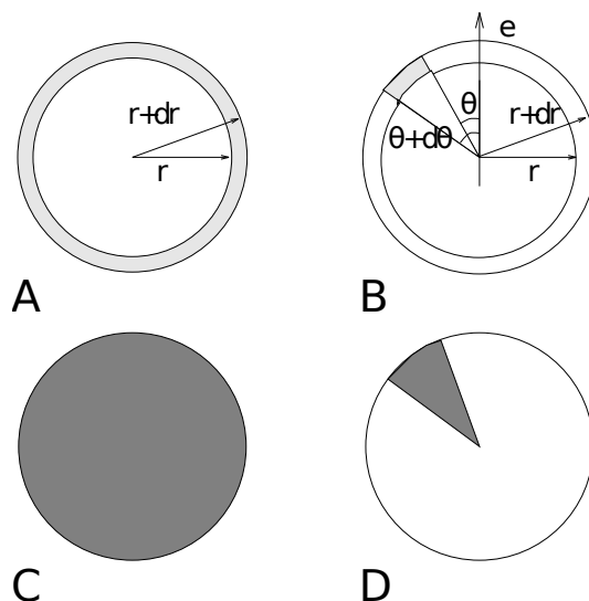
Fig. 5.52: Definition of slices in gmx rdf (page 242): A. g_{AB}(r) . B. g_{AB}(r, \theta) . The slices are colored gray. C. Normalization \langle \rho_B \rangle_{local} . D. Normalization \langle \rho_B \rangle_{local, \theta} . Normalization volumes are colored gray.
