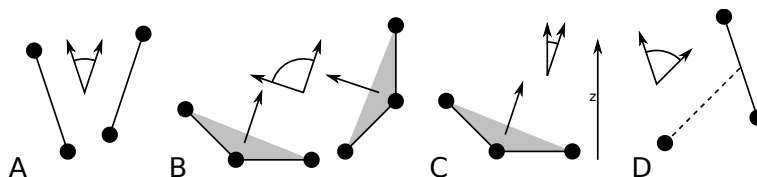
Fig. 5.56: Angle options of gmx gangle (page 184): A. Angle between two vectors. B. Angle between two planes. C. Angle between a vector and the z axis. D. Angle between a vector and the normal of a sphere. Also other combinations are supported: planes and vectors can be used interchangeably.
